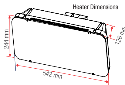
Heater Dimensions
